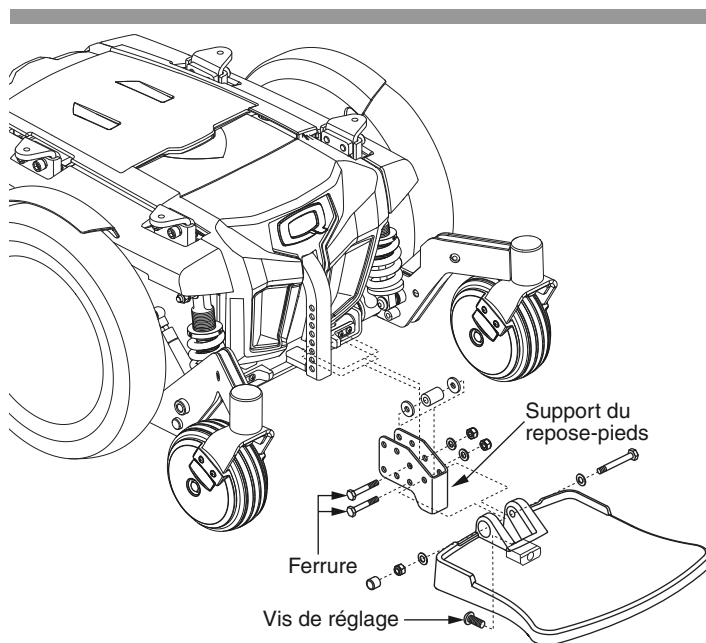
Figure 17. Ajustement de repose-pieds
