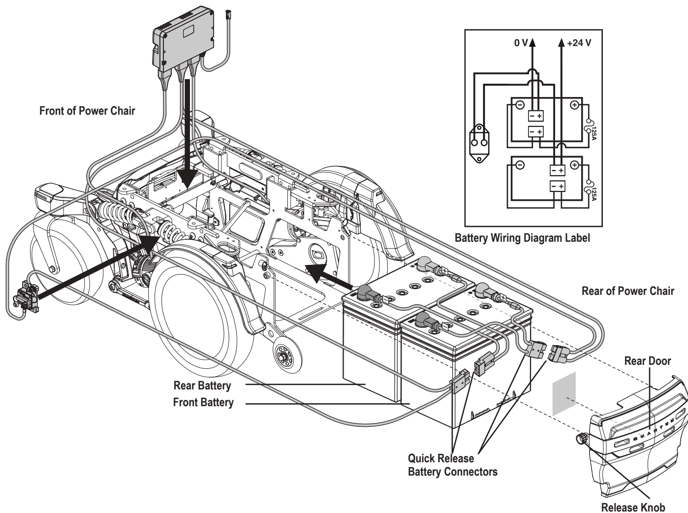
Figure 12. Battery Installation
